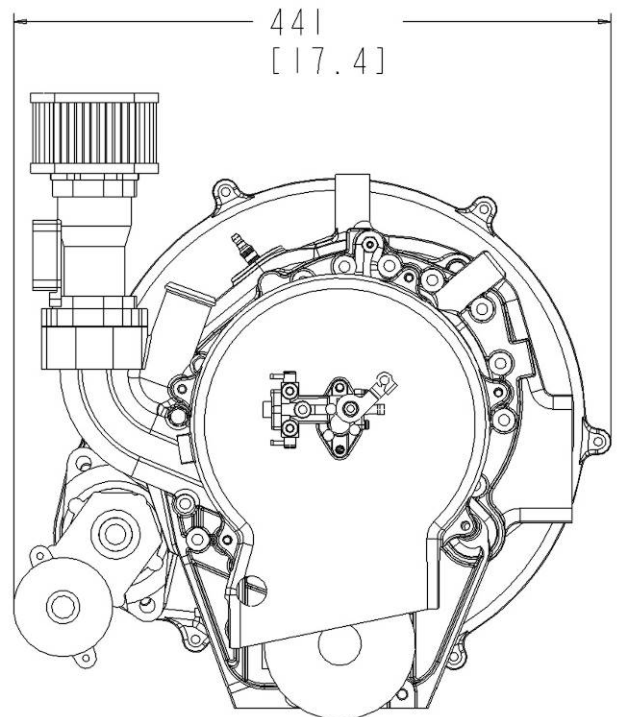
Rotapower 1300 – End View
