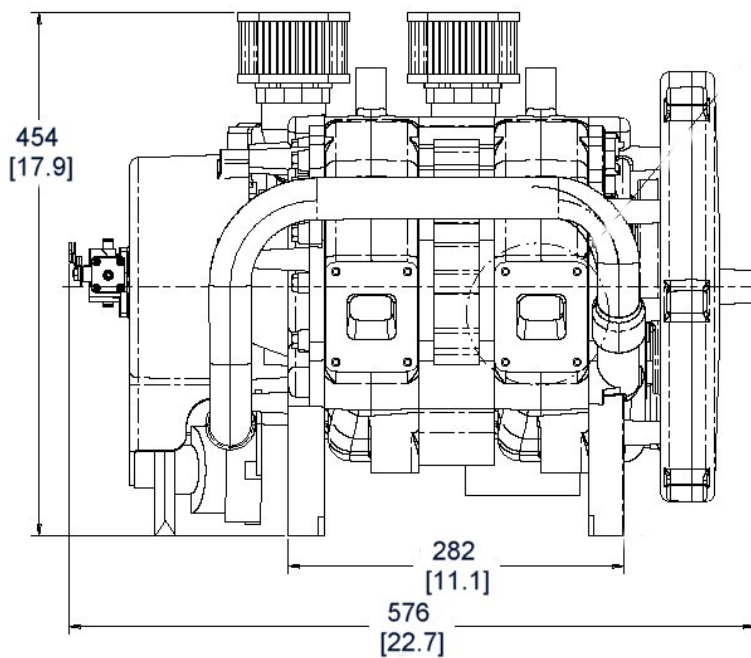
Rotapower 1300 – Side View – Non-compound
