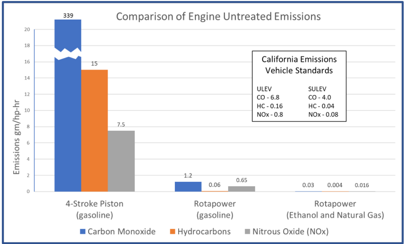
Rotapower® Engine
