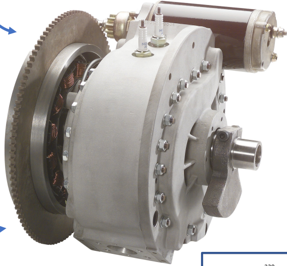
Rotapower® Engine
