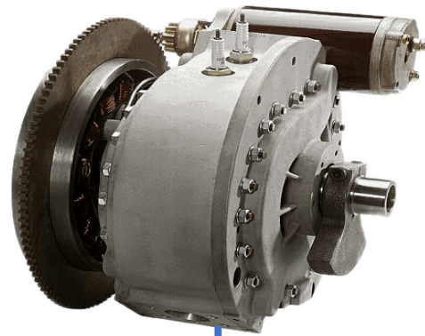
Rotapower® Generator
